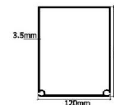
Main frame profile
